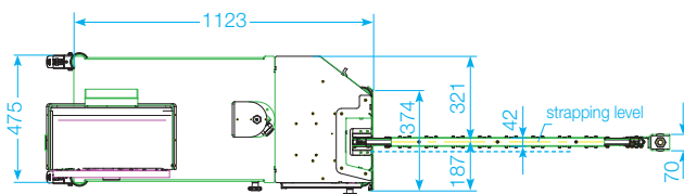
Layout SoniXs MS-6 KR (800 mm x 1600 mm)
